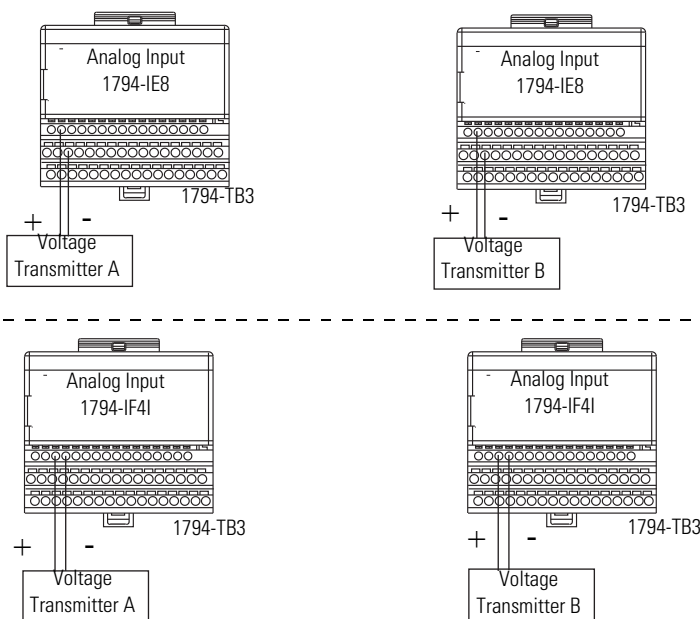
Figure 3.9 FLEX I/O Analog Input Module Wiring in Voltage Mode
